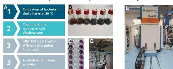
Fig. 2: A: Work-flow for LEEI of bioleaching bacteria [4]; B, C: Cultivation flasks and iron assay; D, E: LEEI facility REAMODE (Reactive Modification with Electrons) and static module.
