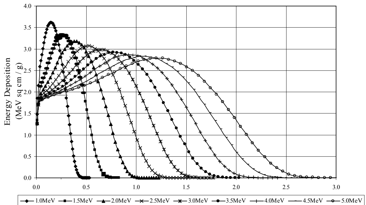
Figure 4. Energy Deposition in Centimeters of Water for 1.0 to 5.0 MeV EB
