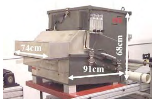
Figure 37. 50cm Two Module Unit Shielded
