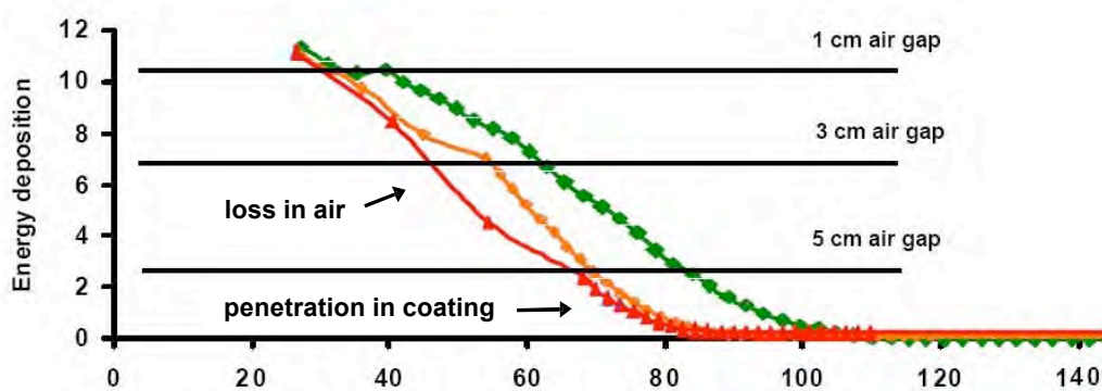
Figure 60. Loss of 80 keV Electron Beam Energy in Air with Change in Gap Distance, Penetration Measured in \mu\text{m} Unit Density
